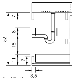
BASE 40 3 + LIVORNO
