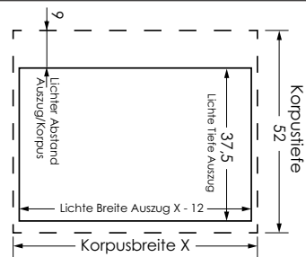
BASE 52
